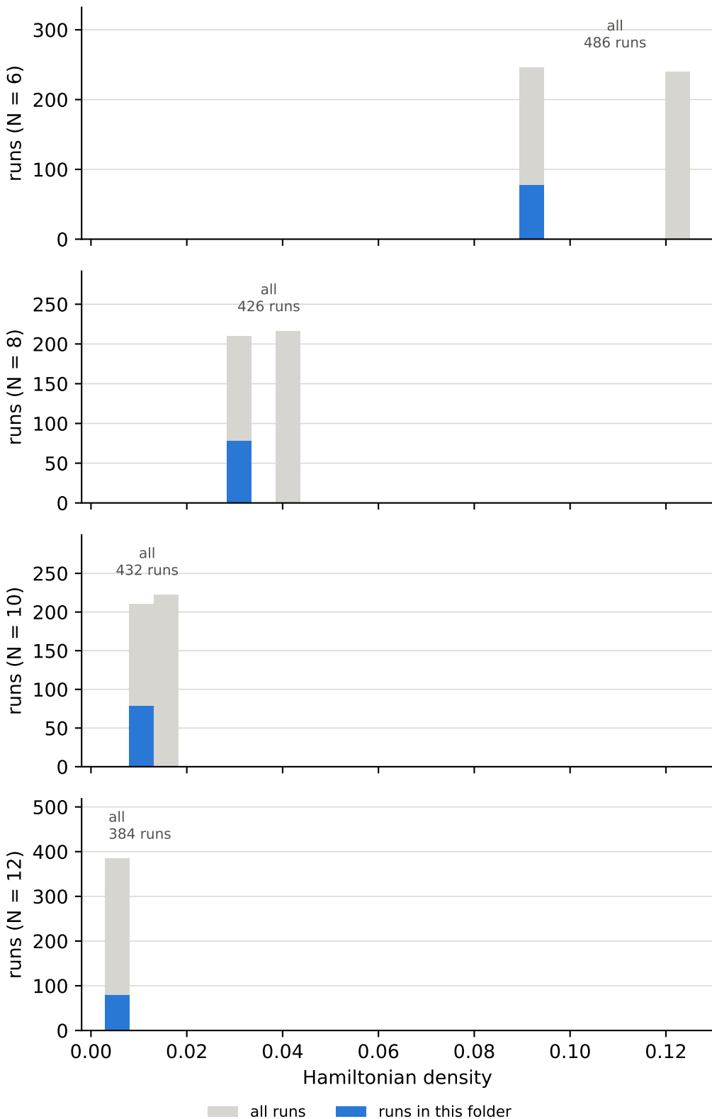
Hamiltonian density over all runs, and the cuts behind the bins lattice dimension = 1, anisotropy \delta = 0
