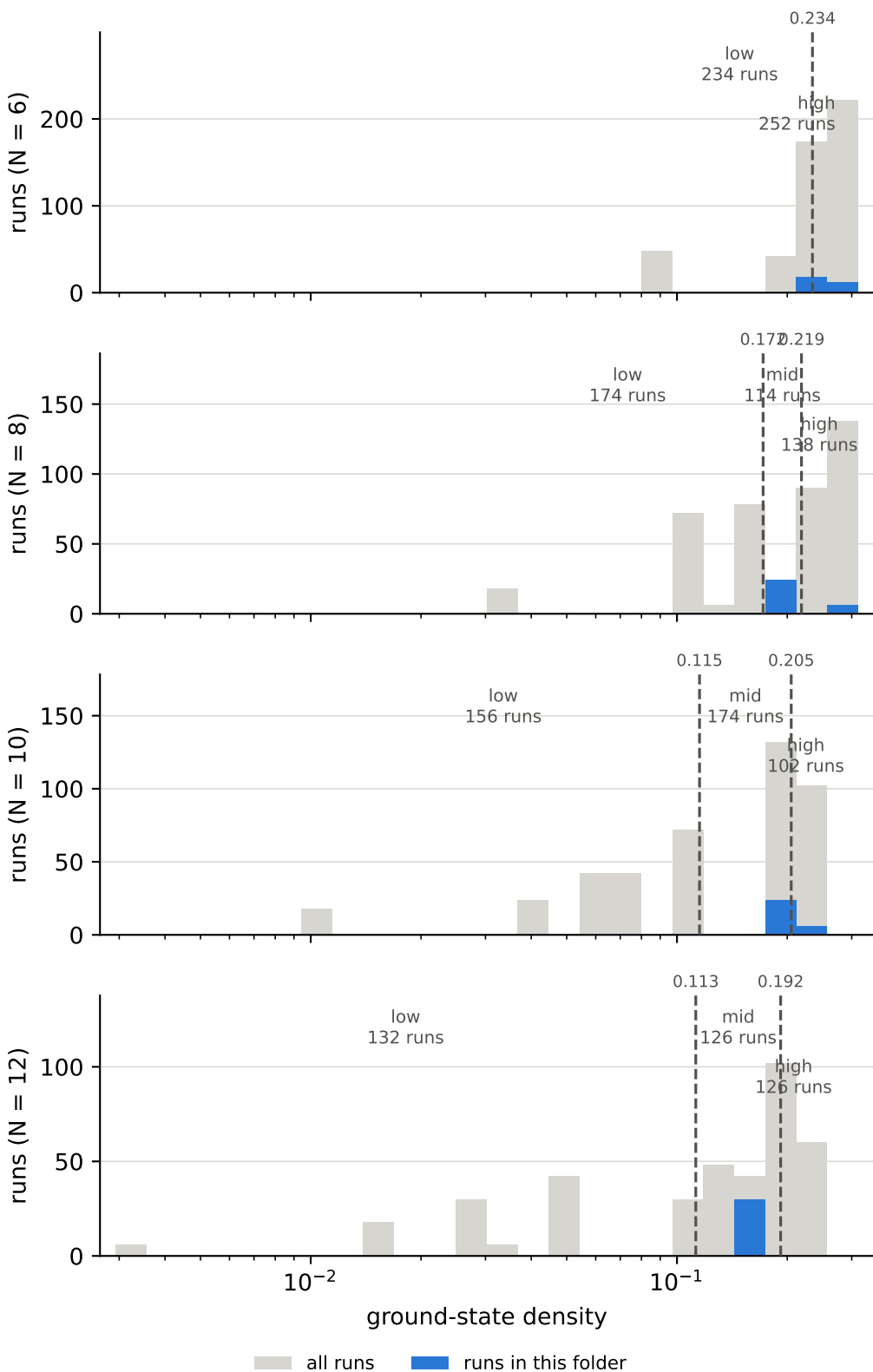
ground-state density over all runs, and the cuts behind the bins lattice dimension = 1, anisotropy \delta = 1
