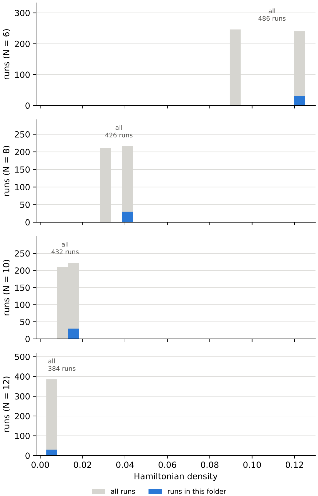
Hamiltonian density over all runs, and the cuts behind the bins lattice dimension = 2, anisotropy delta = 1
