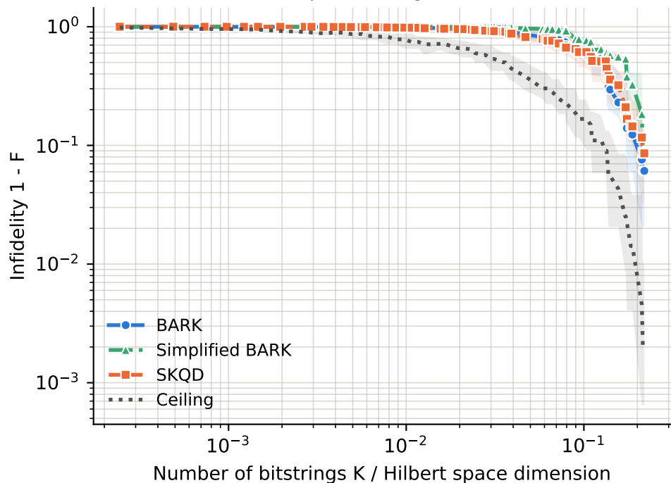
runs per point -- BARK: 18-72, Ceiling: 18-72, SKQD: 18-72, Simplified BARK: 18-72
