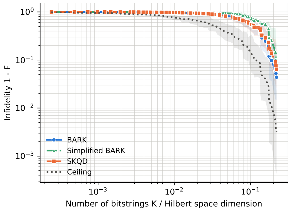
runs per point -- BARK: 18-72, Ceiling: 18-72, SKQD: 18-72, Simplified BARK: 18-72
