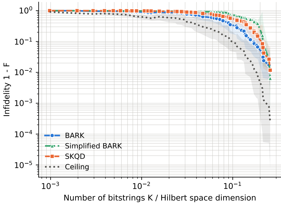
runs per point -- BARK: 6-24, Ceiling: 6-24, SKQD: 6-24, Simplified BARK: 6-24
