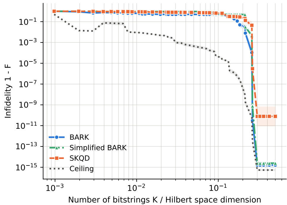
runs per point -- BARK: 18-36, Ceiling: 18-36, SKQD: 18-36, Simplified BARK: 18-36
