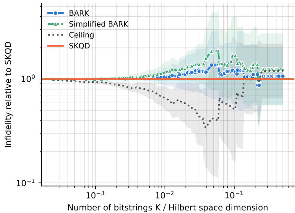
runs per point -- BARK: 8-34, Ceiling: 8-34, SKQD: 8-34, Simplified BARK: 8-34
