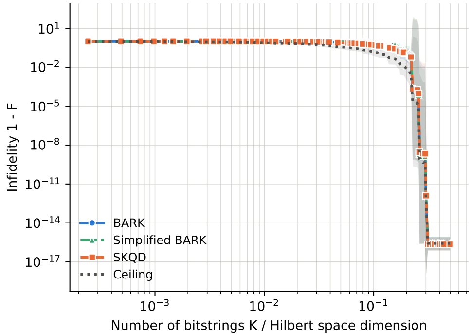
runs per point -- BARK: 6-34, Ceiling: 6-34, SKQD: 6-34, Simplified BARK: 6-34
