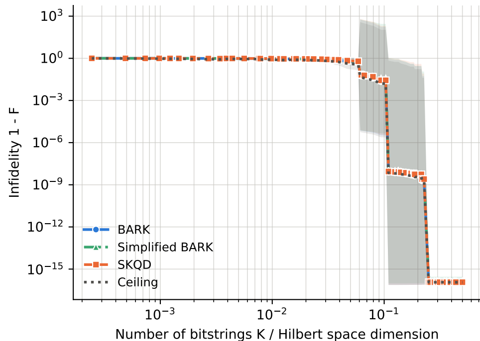
runs per point -- BARK: 1-16, Ceiling: 1-16, SKQD: 1-16, Simplified BARK: 1-16
