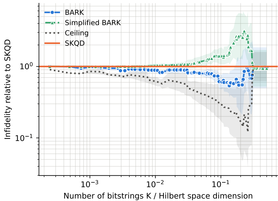
runs per point -- BARK: 2-19, Ceiling: 2-19, SKQD: 2-19, Simplified BARK: 2-19
