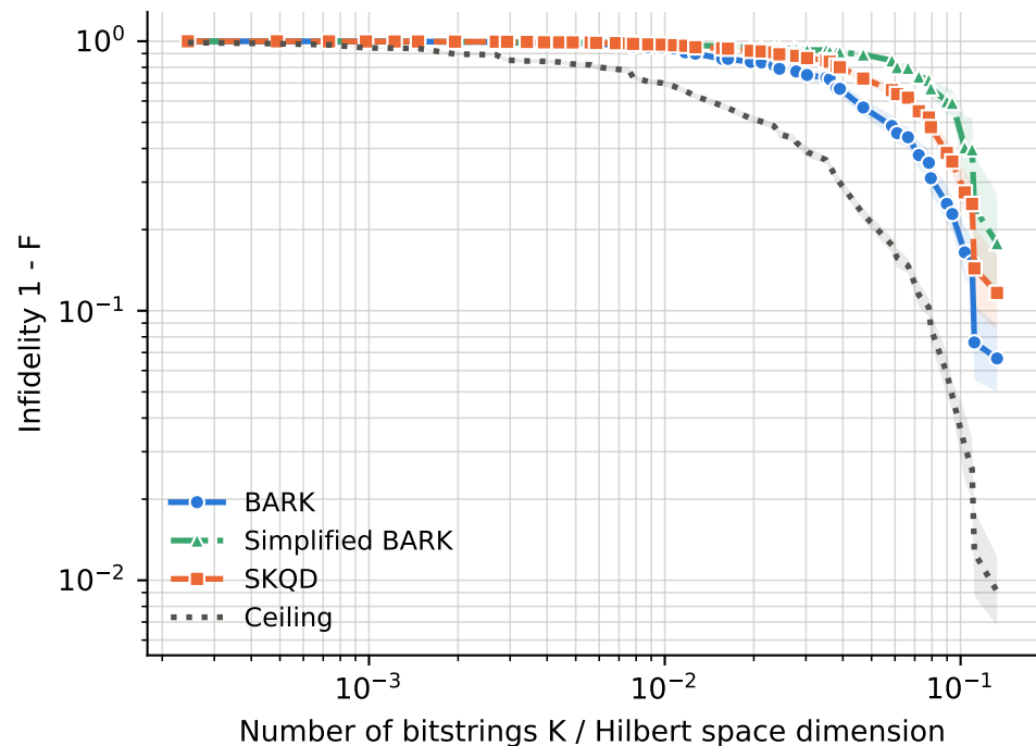
runs per point -- BARK: 3-18, Ceiling: 3-18, SKQD: 3-18, Simplified BARK: 3-18
