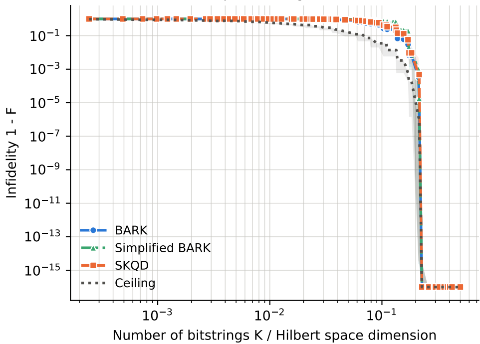
runs per point -- BARK: 4-10, Ceiling: 4-10, SKQD: 4-10, Simplified BARK: 4-10
