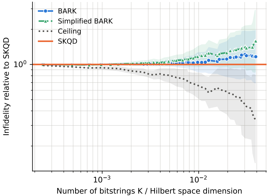
runs per point -- BARK: 8-34, Ceiling: 8-34, SKQD: 8-34, Simplified BARK: 8-34
