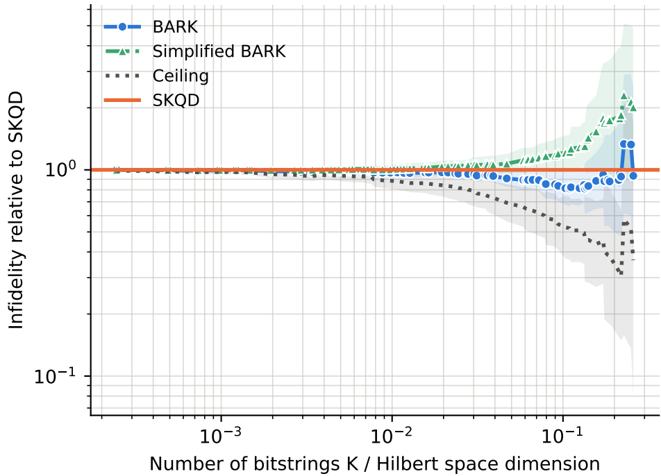
runs per point -- BARK: 3-23, Ceiling: 3-23, SKQD: 3-23, Simplified BARK: 3-23
