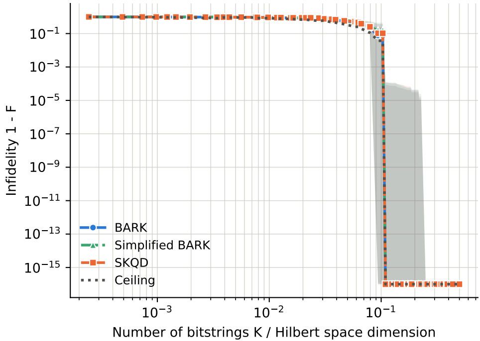
runs per point -- BARK: 5-38, Ceiling: 5-38, SKQD: 5-38, Simplified BARK: 5-38
