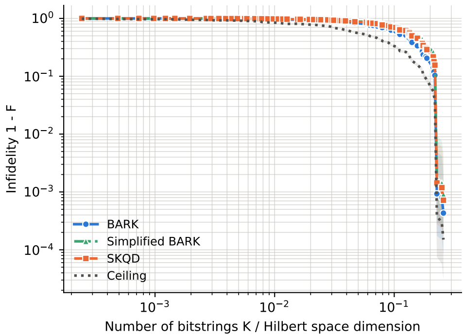
runs per point -- BARK: 7-51, Ceiling: 7-51, SKQD: 7-51, Simplified BARK: 7-51
