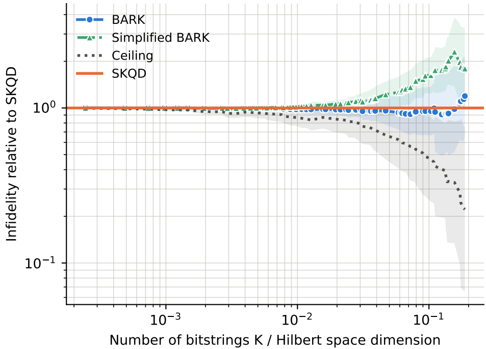
runs per point -- BARK: 4-35, Ceiling: 4-35, SKQD: 4-35, Simplified BARK: 4-35
