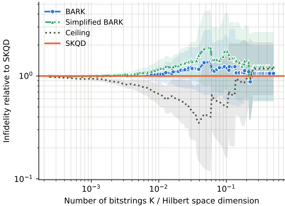
runs per point -- BARK: 8-36, Ceiling: 8-36, SKQD: 8-36, Simplified BARK: 8-36
