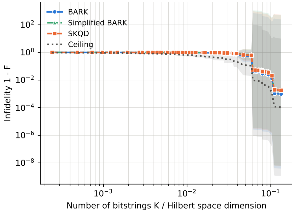
runs per point -- BARK: 8-14, Ceiling: 8-14, SKQD: 8-14, Simplified BARK: 8-14
