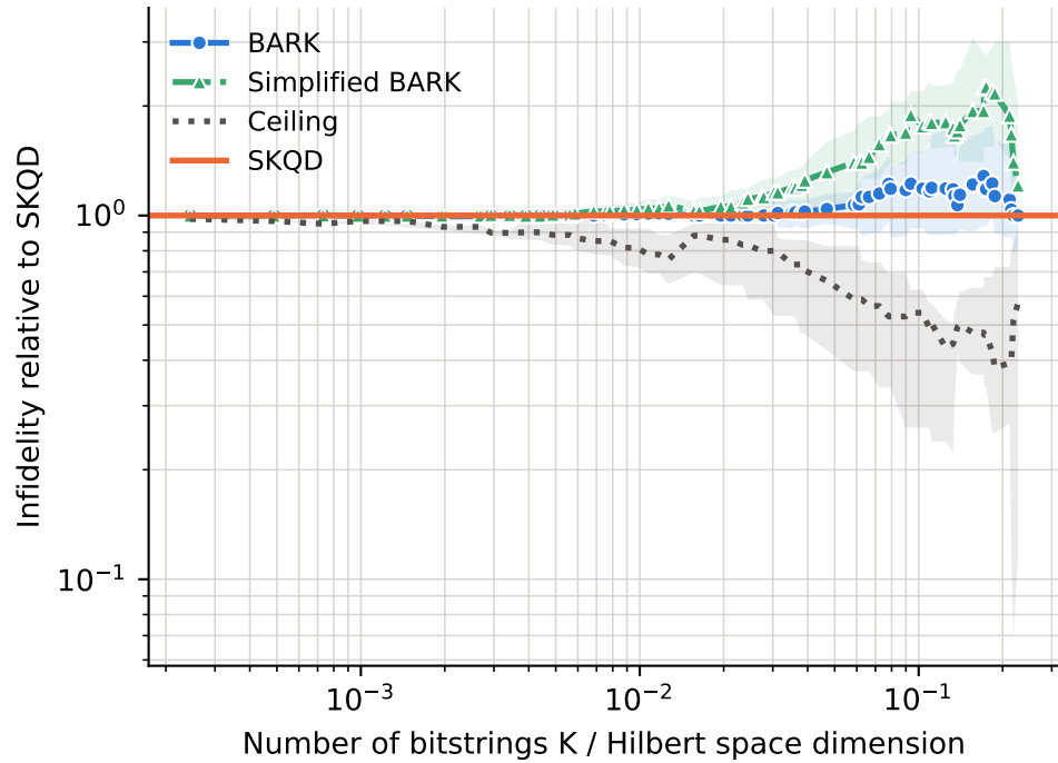
runs per point -- BARK: 5-36, Ceiling: 5-36, SKQD: 5-36, Simplified BARK: 5-36
