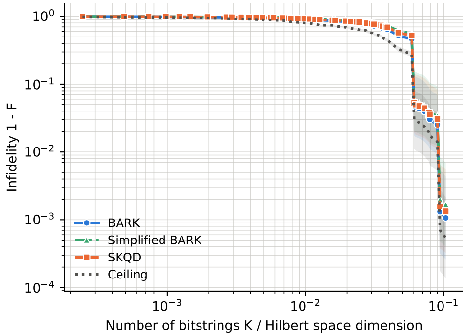
runs per point -- BARK: 19-77, Ceiling: 19-77, SKQD: 19-77, Simplified BARK: 19-77
