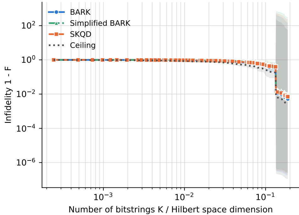
runs per point -- BARK: 9-43, Ceiling: 9-43, SKQD: 9-43, Simplified BARK: 9-43
