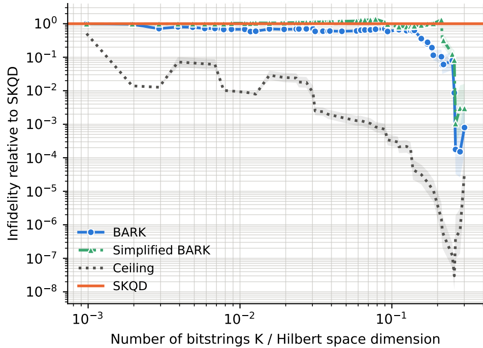
runs per point -- BARK: 16-47, Ceiling: 16-47, SKQD: 16-47, Simplified BARK: 16-47
