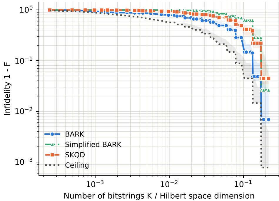
runs per point -- BARK: 4-6, Ceiling: 4-6, SKQD: 4-6, Simplified BARK: 4-6
