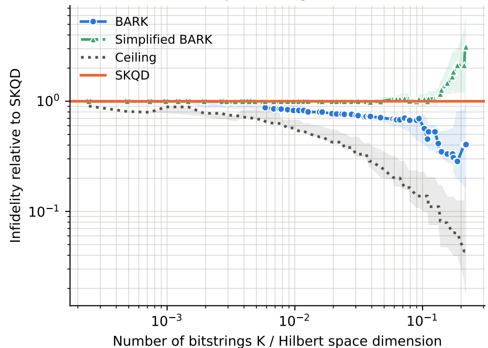
runs per point -- BARK: 3-15, Ceiling: 3-15, SKQD: 3-15, Simplified BARK: 3-15
