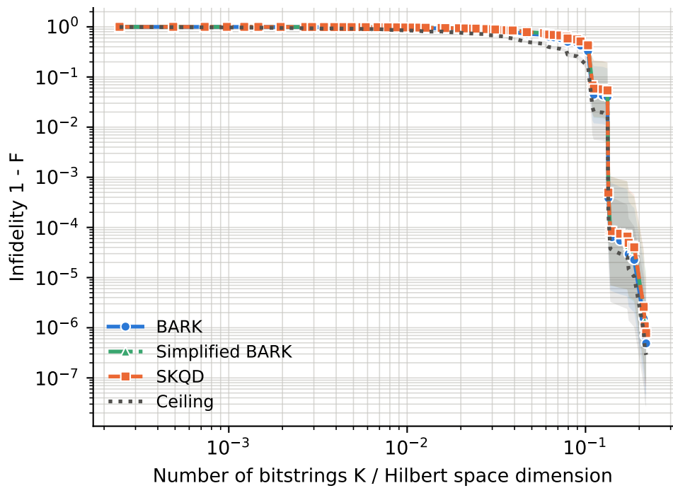
runs per point -- BARK: 14-38, Ceiling: 14-38, SKQD: 14-38, Simplified BARK: 14-38
