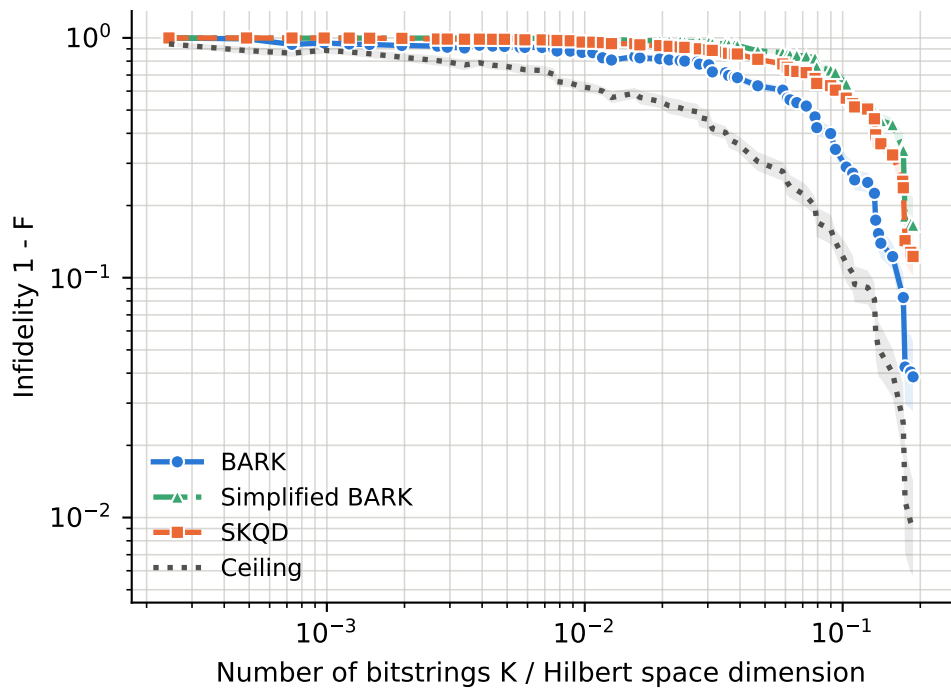
runs per point -- BARK: 5-16, Ceiling: 5-16, SKQD: 5-16, Simplified BARK: 5-16
