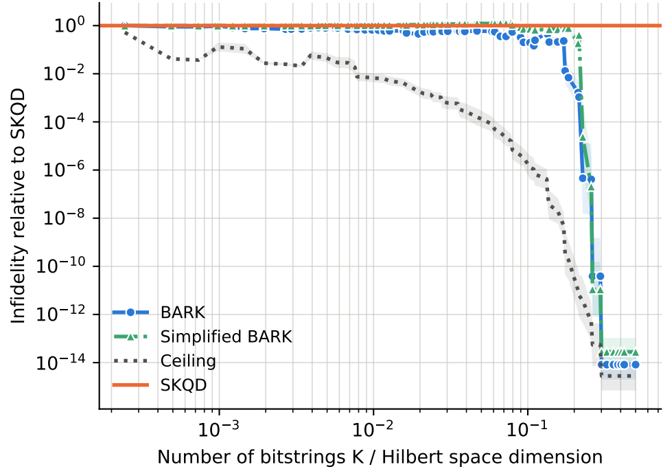
runs per point -- BARK: 6-18, Ceiling: 6-18, SKQD: 6-18, Simplified BARK: 6-18
