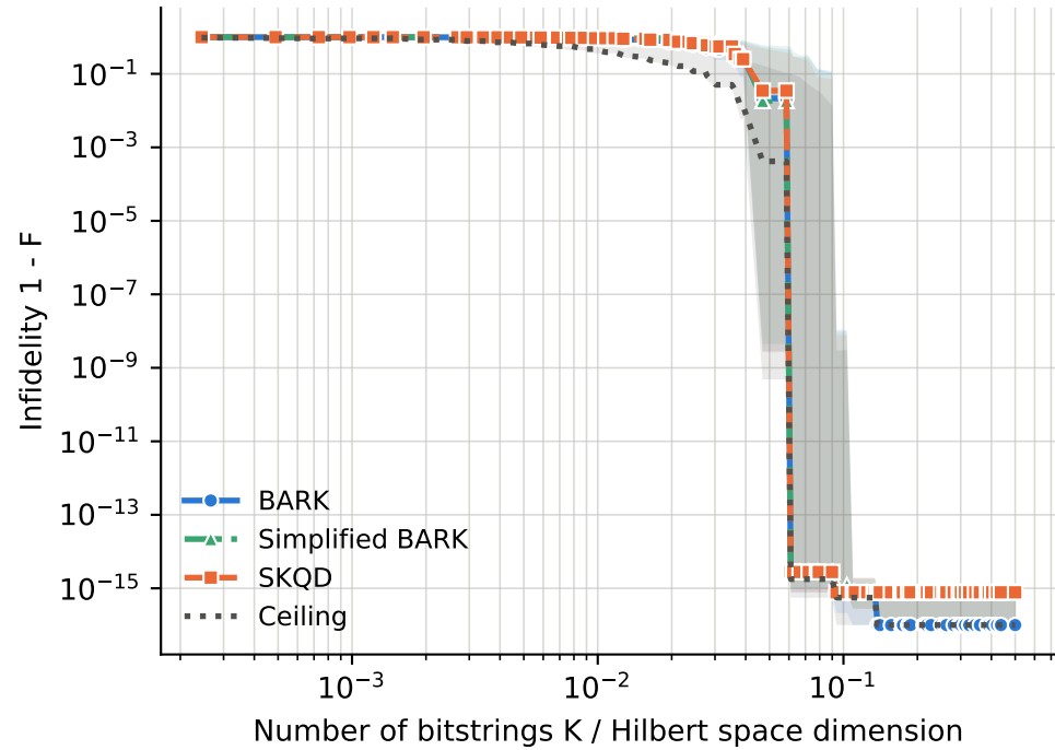
runs per point -- BARK: 3-11, Ceiling: 3-11, SKQD: 3-11, Simplified BARK: 3-11
