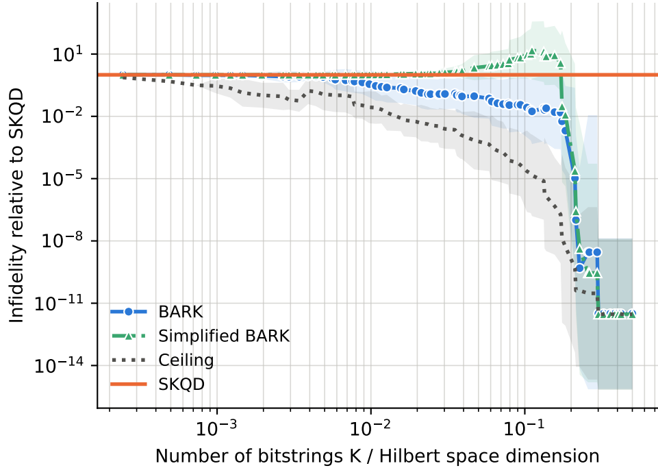
runs per point -- BARK: 6-23, Ceiling: 6-23, SKQD: 6-23, Simplified BARK: 6-23
