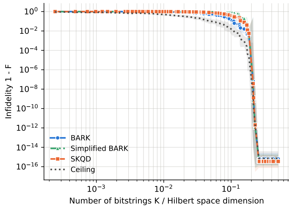
runs per point -- BARK: 2-8, Ceiling: 2-8, SKQD: 2-8, Simplified BARK: 2-8
