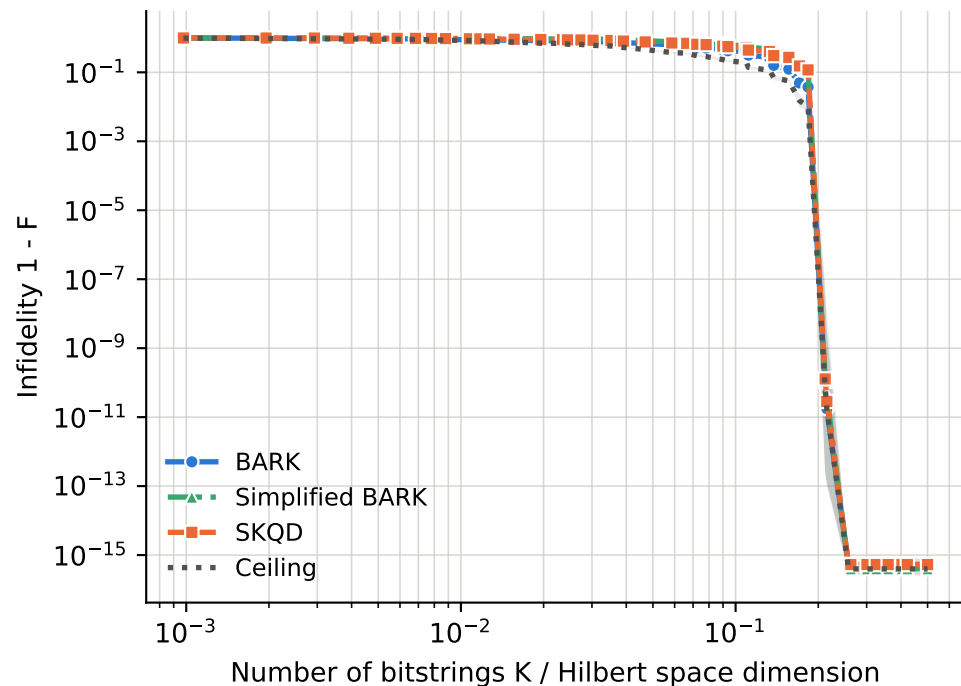
runs per point -- BARK: 5-8, Ceiling: 5-8, SKQD: 5-8, Simplified BARK: 5-8
