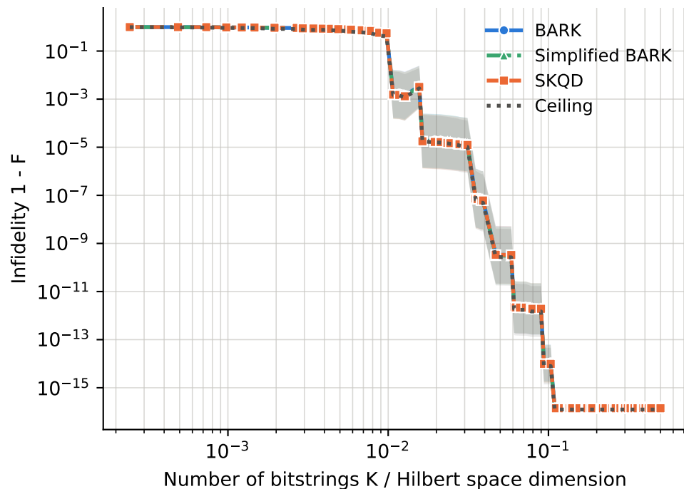
runs per point -- BARK: 12-41, Ceiling: 12-41, SKQD: 12-41, Simplified BARK: 12-41
