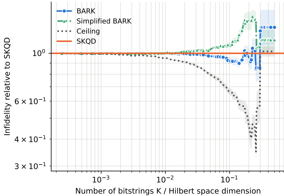
runs per point -- BARK: 1-12, Ceiling: 1-12, SKQD: 1-12, Simplified BARK: 1-12
