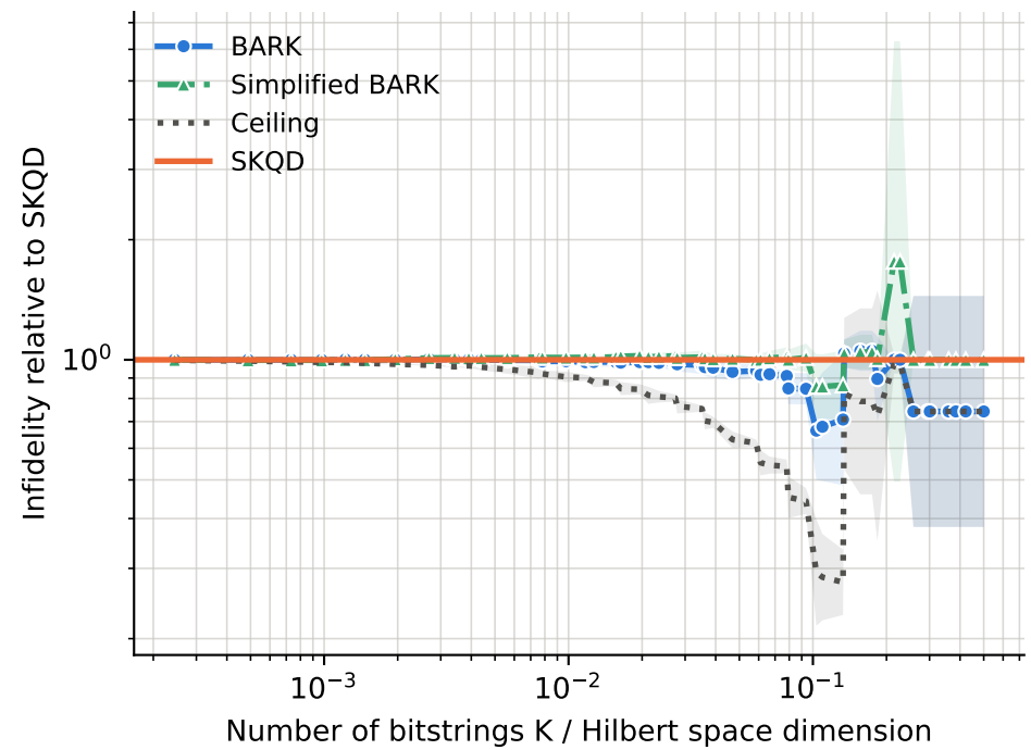
runs per point -- BARK: 4-5, Ceiling: 4-5, SKQD: 4-5, Simplified BARK: 4-5
