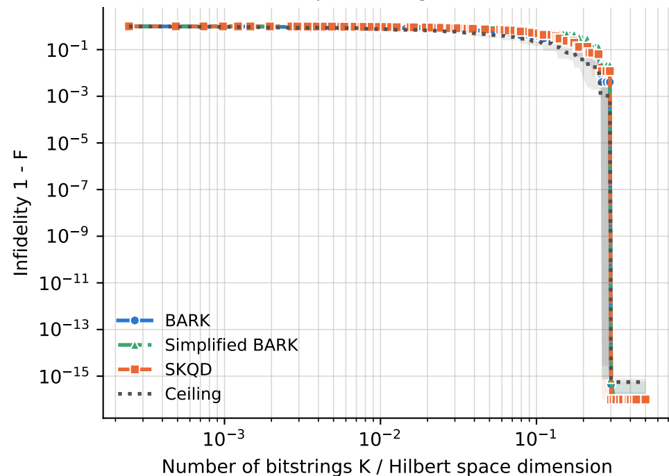
runs per point -- BARK: 2-11, Ceiling: 2-11, SKQD: 2-11, Simplified BARK: 2-11
