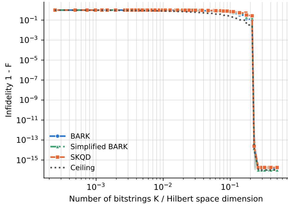
runs per point -- BARK: 6-7, Ceiling: 6-7, SKQD: 6-7, Simplified BARK: 6-7
