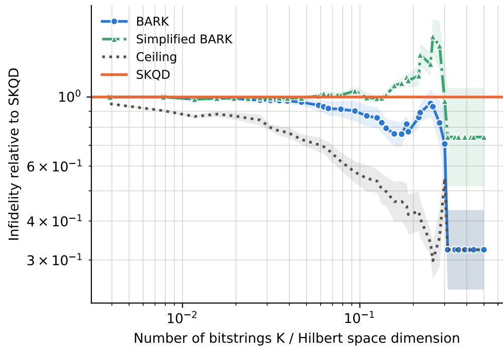
runs per point -- BARK: 3-7, Ceiling: 3-7, SKQD: 3-7, Simplified BARK: 3-7
