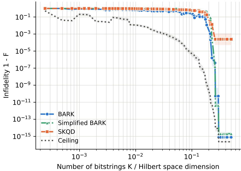
runs per point -- BARK: 5-27, Ceiling: 5-27, SKQD: 5-27, Simplified BARK: 5-27
