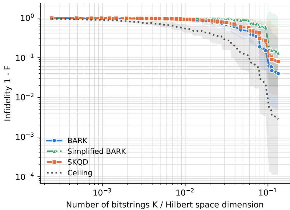
runs per point -- BARK: 12-36, Ceiling: 12-36, SKQD: 12-36, Simplified BARK: 12-36
