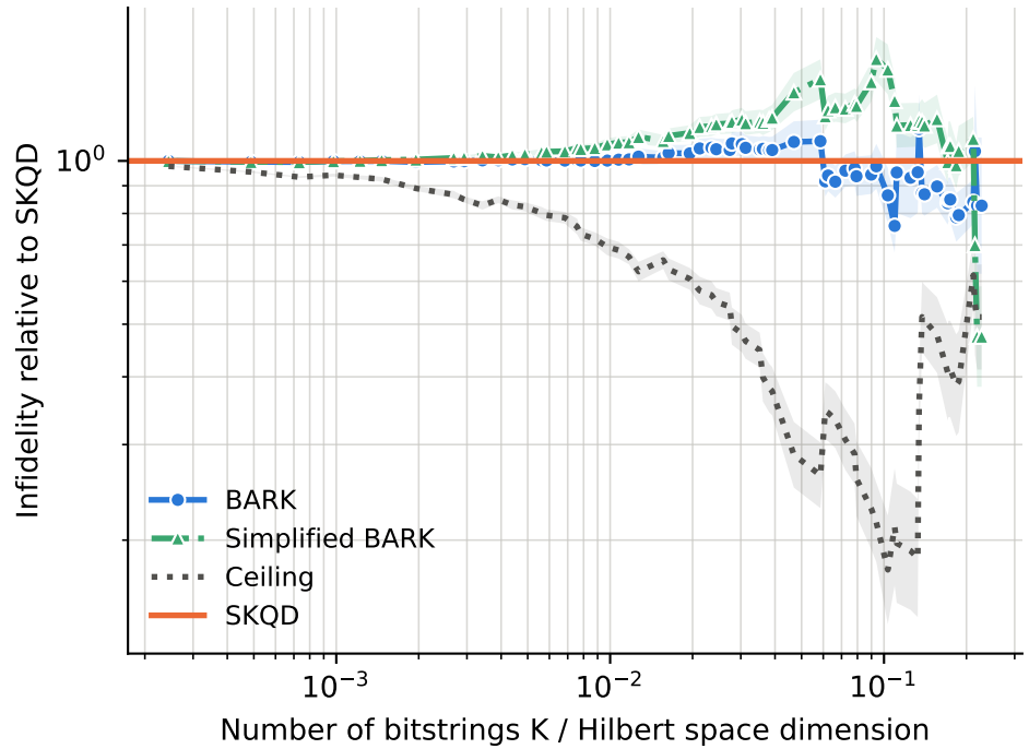
runs per point -- BARK: 12-48, Ceiling: 12-48, SKQD: 12-48, Simplified BARK: 12-48
