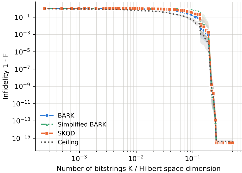
runs per point -- BARK: 1-13, Ceiling: 1-13, SKQD: 1-13, Simplified BARK: 1-13
