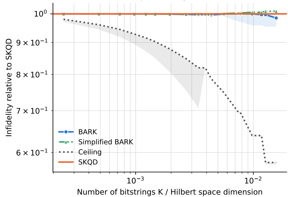
runs per point -- BARK: 4-5, Ceiling: 4-5, SKQD: 4-5, Simplified BARK: 4-5
