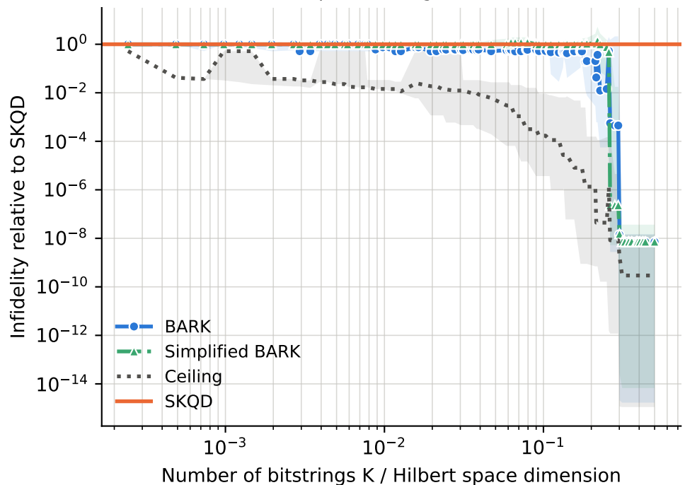
runs per point -- BARK: 5-39, Ceiling: 5-39, SKQD: 5-39, Simplified BARK: 5-39
