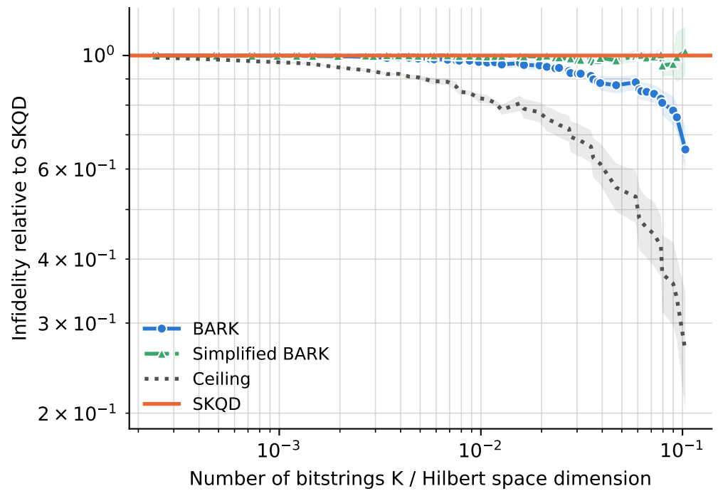
runs per point -- BARK: 3-8, Ceiling: 3-8, SKQD: 3-8, Simplified BARK: 3-8
