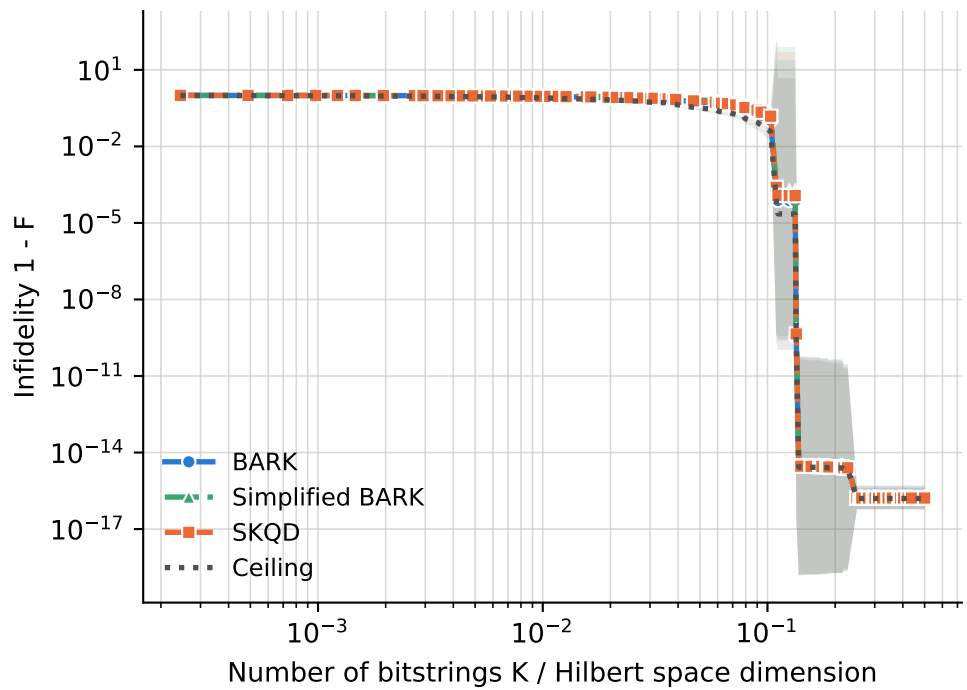
runs per point -- BARK: 9-25, Ceiling: 9-25, SKQD: 9-25, Simplified BARK: 9-25
