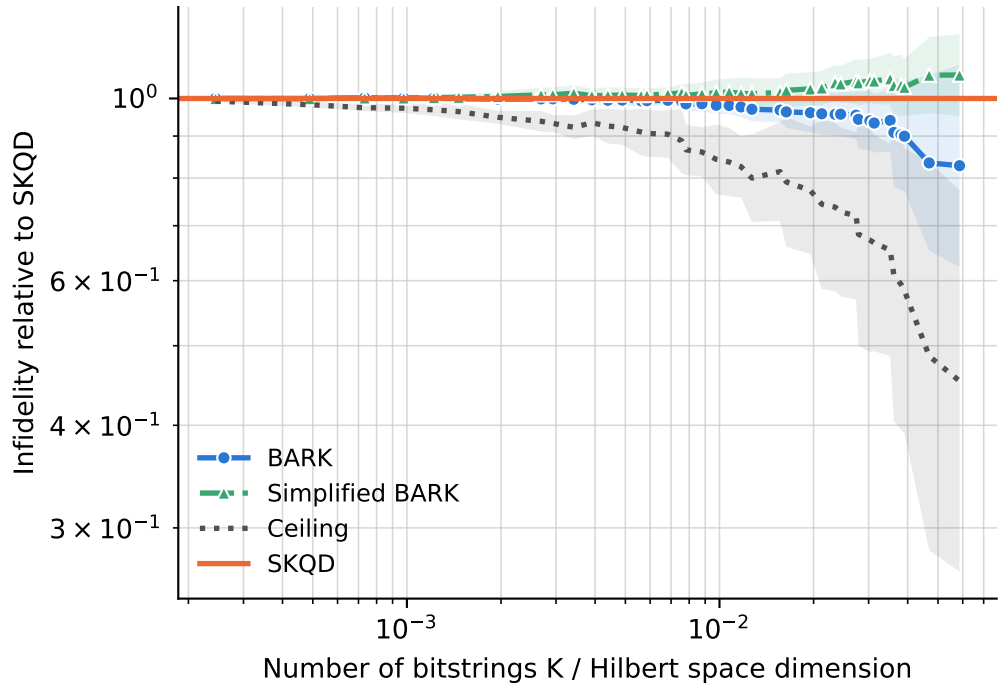
runs per point -- BARK: 7-24, Ceiling: 7-24, SKQD: 7-24, Simplified BARK: 7-24
