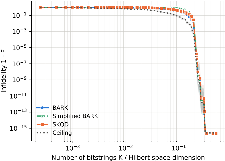
runs per point -- BARK: 2-16, Ceiling: 2-16, SKQD: 2-16, Simplified BARK: 2-16
