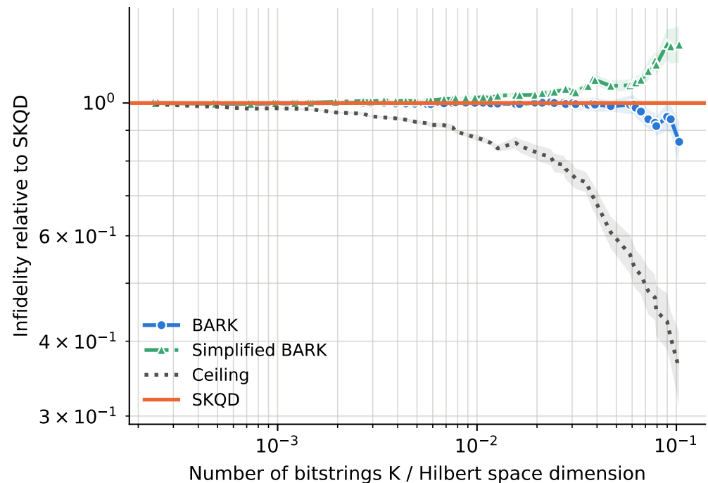
runs per point -- BARK: 3-16, Ceiling: 3-16, SKQD: 3-16, Simplified BARK: 3-16
